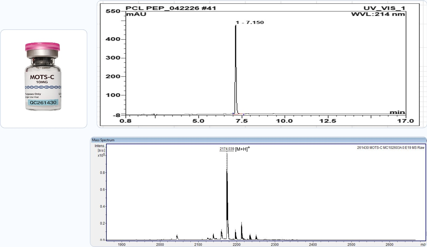
HPLC Chromatogram (Retention Time: 7.150 min)
