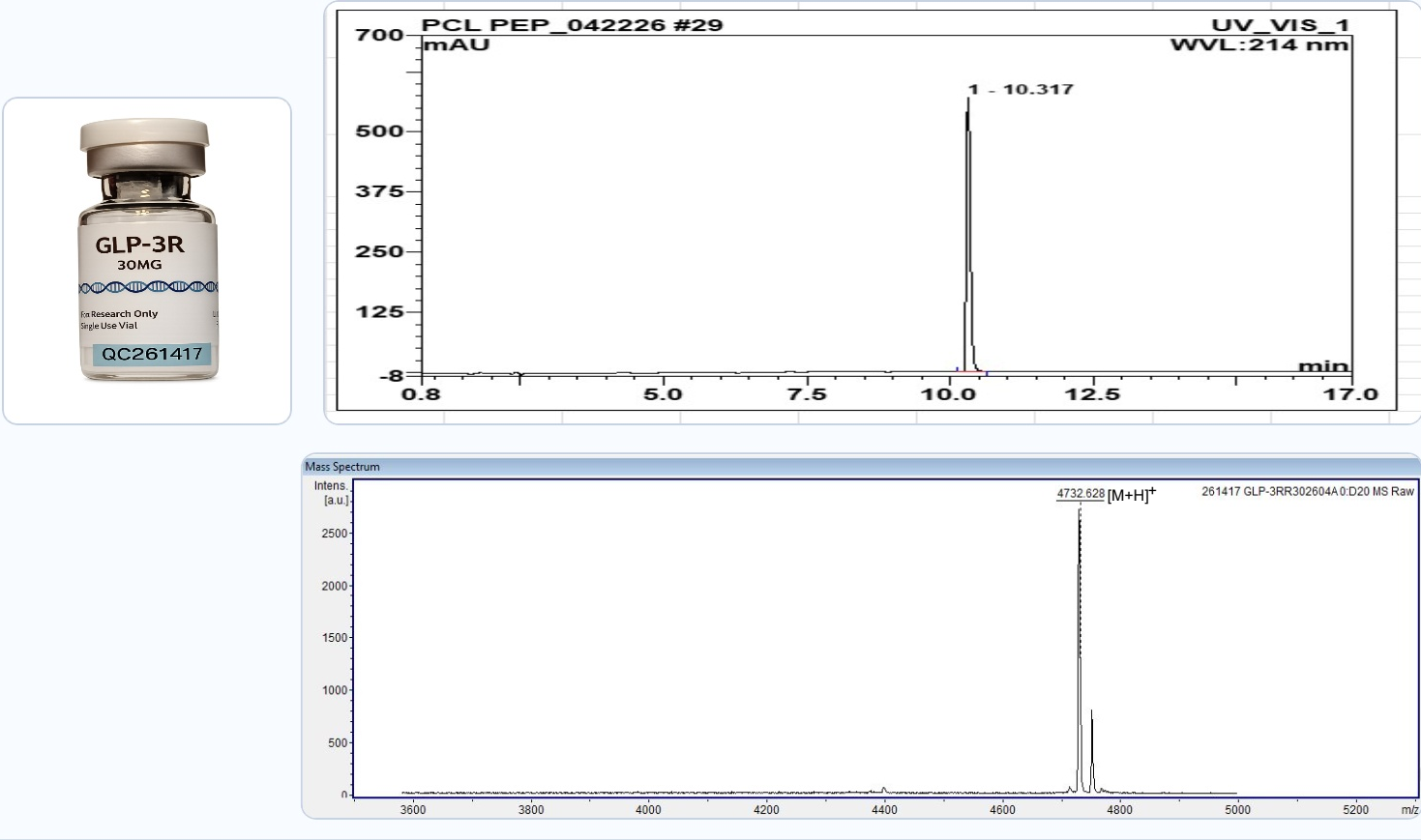
HPLC Chromatogram (Retention Time: 10.317 min)
