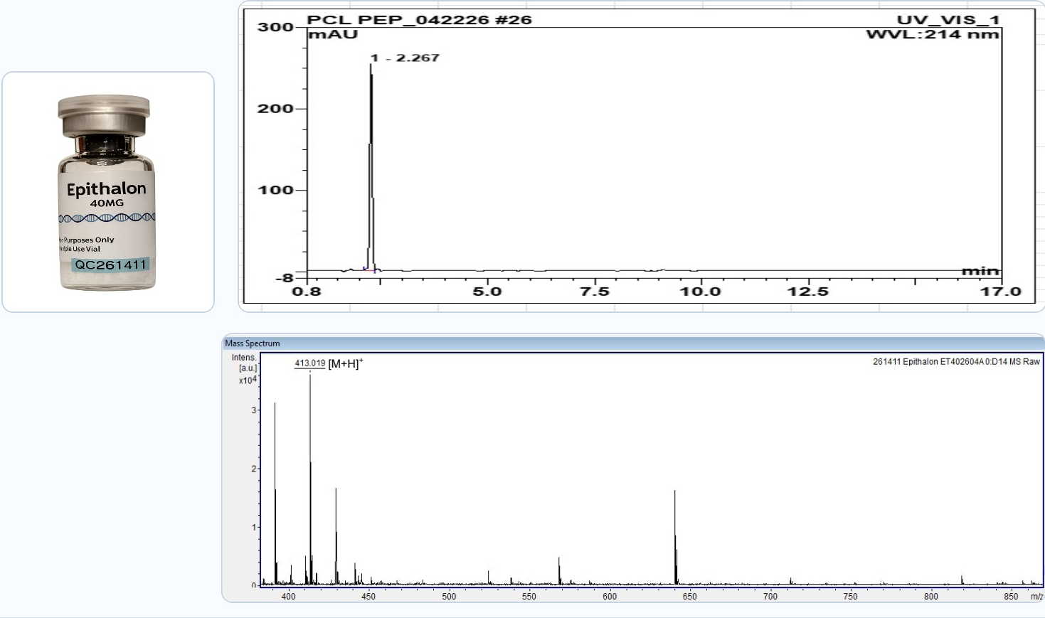
HPLC Chromatogram (Retention Time: 2.267 min)
