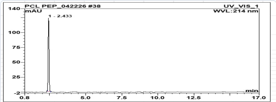
HPLC Chromatogram (Retention Time: 2.433 min)
