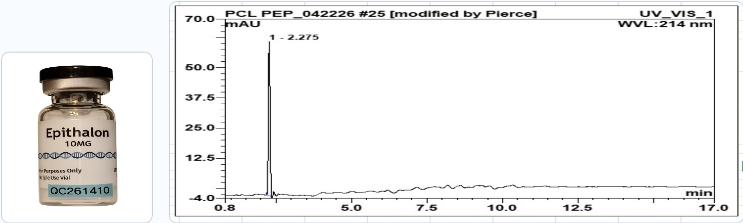
HPLC Chromatogram (Retention Time: 2.275 min)
