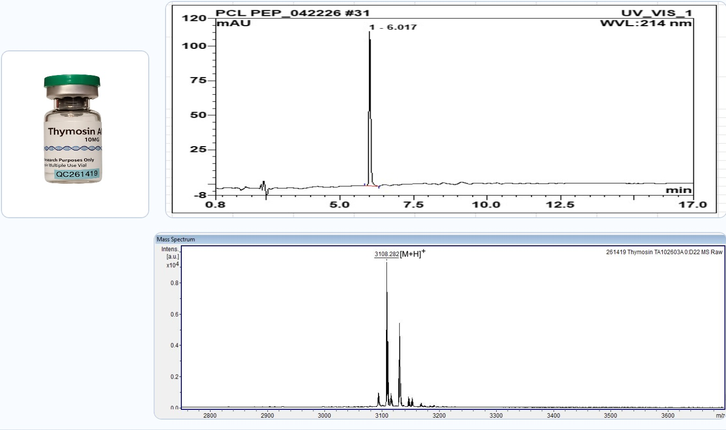
HPLC Chromatogram (Retention Time: 6.017 min)
